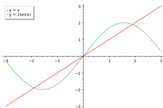
Figure 1: The equation x = 2\sin(x) has exactly three solutions. This SageMath-generated plot shows that these solutions are x = 0 (exactly) and x \approx \pm 1.89 .
