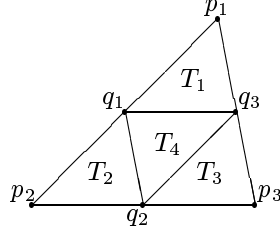
FIGURE 5. A Triangle T \in \mathcal{T}_{k-1} divided into four triangles in \mathcal{T}_k
