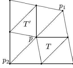
FIGURE 4. A vertex p \in \mathcal{T}_k \setminus \mathcal{T}_{k-1}
