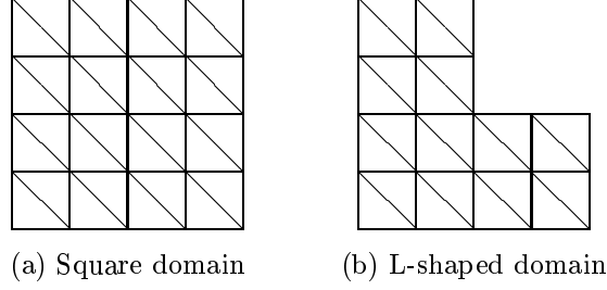
FIGURE 6. The triangulation \mathcal{T}_k for k = 2 .
