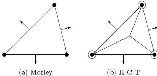
FIGURE 1. The Morley element and the H-C-T element
