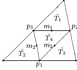
FIGURE 3. A reference triangle \tilde{T} divided into 4 triangles \tilde{T}_1, \tilde{T}_2, \tilde{T}_3 and \tilde{T}_4
