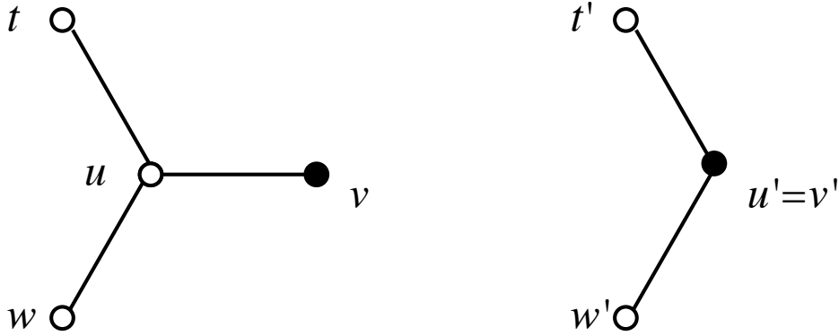
Figure 2: t, u, w \in \overline{X} , v \in X ; t', w' \in \overline{(X')} , u' = v' \in X' . A single edge in E(X, \overline{X}) may correspond to two edges in E(X', \overline{(X')}) .
